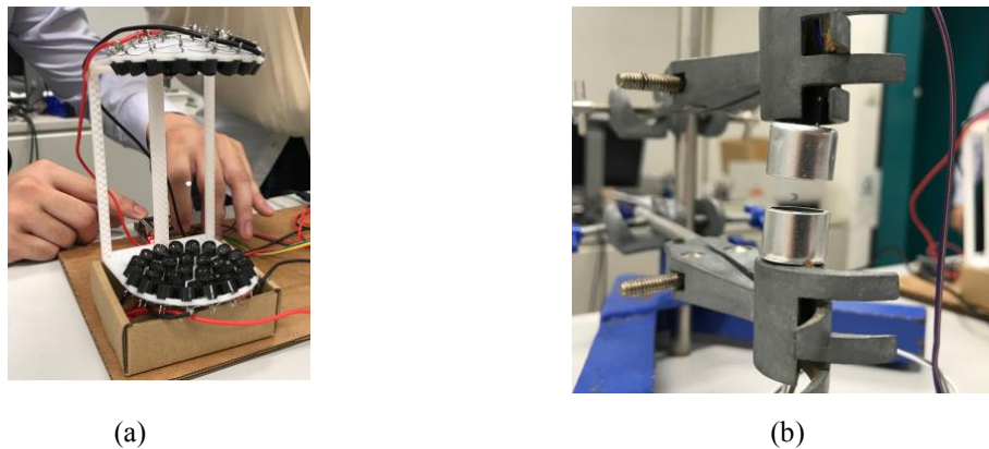
Figure 3. (a) & (b) Setting of experiment of sonic levitation
